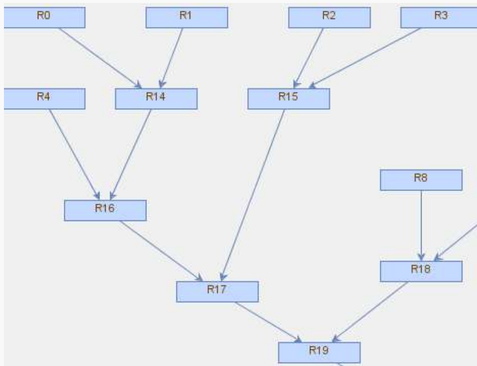
role-permission
